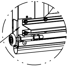
DETAIL D
